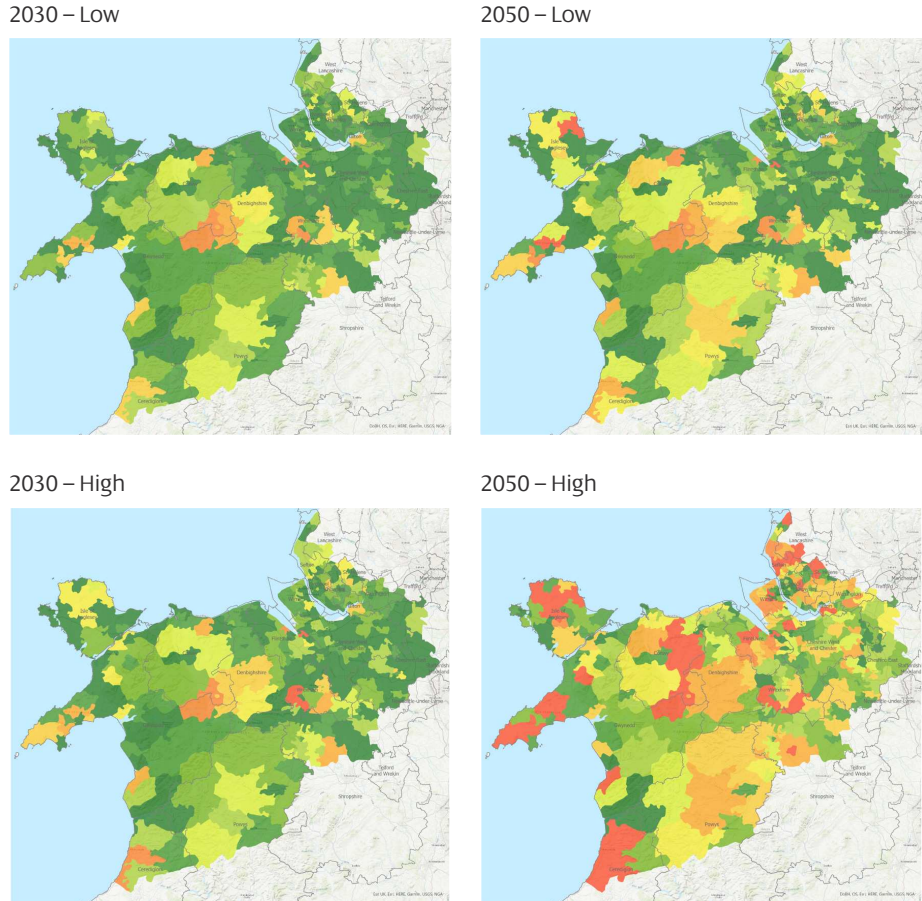
Figure 20 | Domestic-scale and smaller-scale installed generation and storage capacity by primary substation area Scale range: 0MW to >12MW
