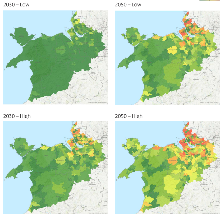
Figure 11 | Residential battery EV uptake numbers by primary substation area Scale range: 0 to >15,000
