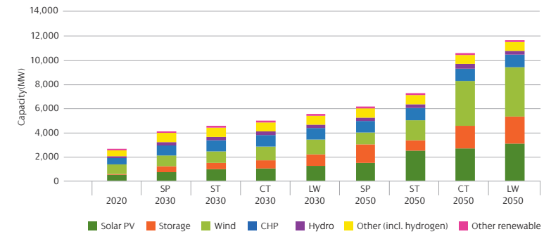
Figure 19 | Installed generation and storage capacity by GSP area
