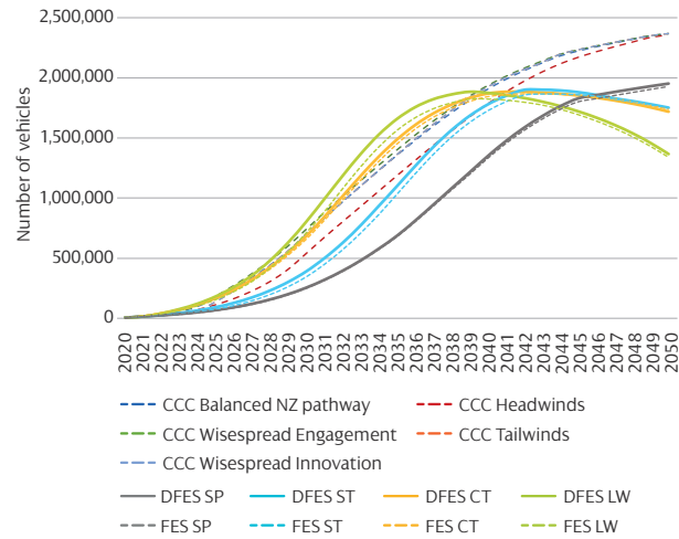
Figure 32 | Battery electric vehicle uptake comparison
