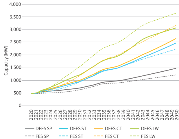
Figure 29 | Solar PV generation capacity comparison (Gen_BB012 and Gen_BB013)
