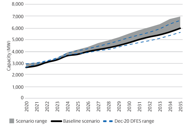
Figure 35 | Range of Net Zero compliant distributed generation forecasts
