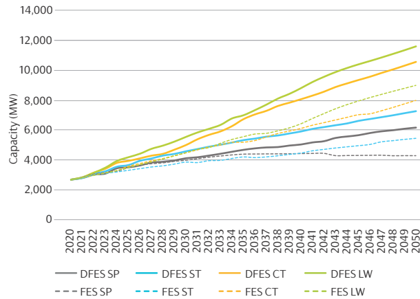
Figure 28 | Distributed generation and storage capacity comparison (Gen_BB001 to Gen_BB023, Srg_BB001 to Srg_BB004)
