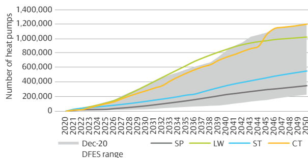
Figure 12 | Electric heat pump uptake
