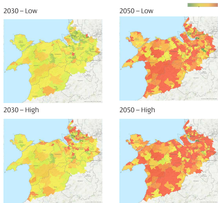
Figure 7 | Electricity peak demand changes from 2020 by primary substation area Scale range: -6MWto >5MW
