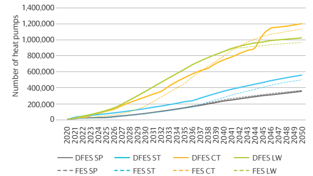
Figure 27 | Heat pump uptake comparison (Lct_BB005 to Lct_BB008)
